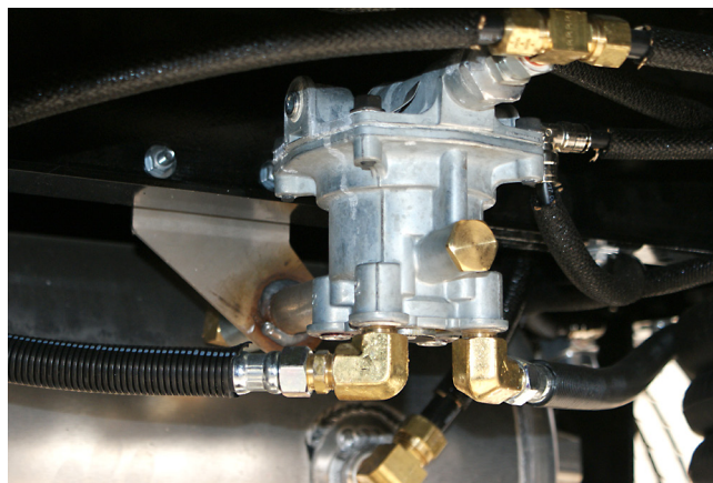
Relay Emergency Valve
