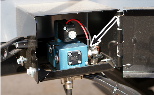
2 Pos, 4 Way MAC Air Valve
