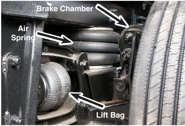
Lift Bag Air Spring Brake Chamber
