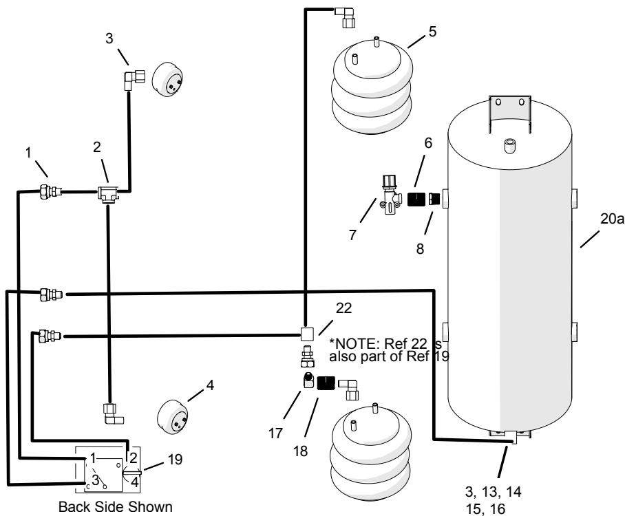
Air Port Identification for REF 19
