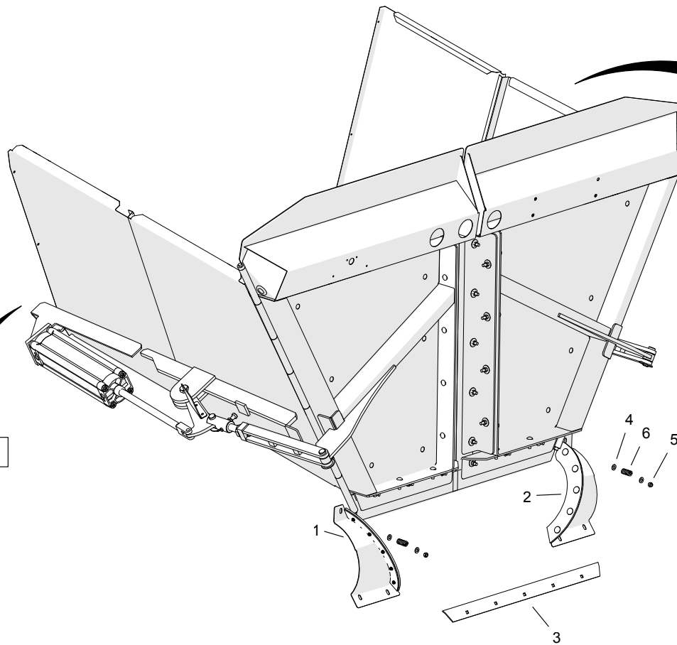
VIEW A- LH SIDE
