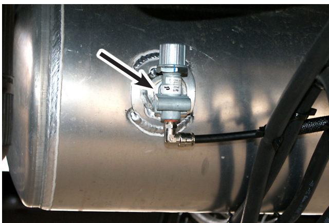
Valve-Pressure Protection Regulator
