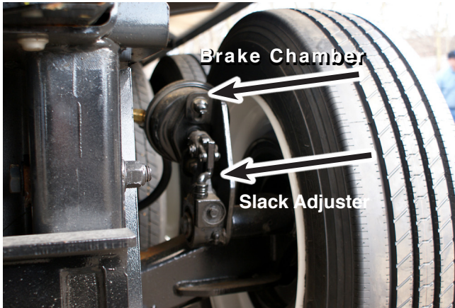
Brake Chamber Slack Adjuster
