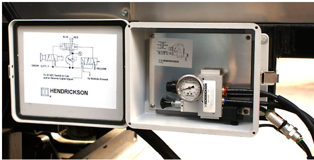
Kit-Air, for Composite
